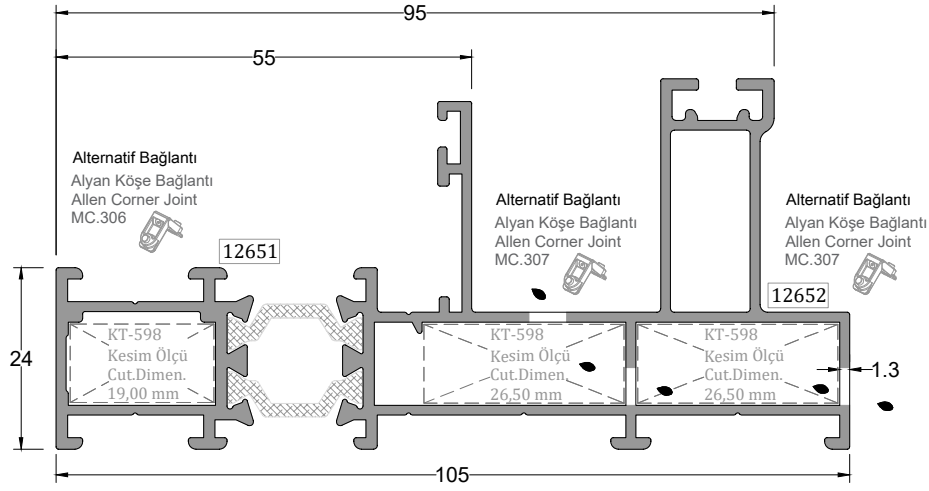
Tek Raylı Kasa Profili MONORAIL FRAME PROFILE
