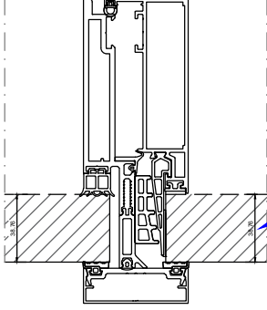
İÇE ÇİFT EKSEN AÇILIM KAPAKLI CEPHE ( TILT&amp;TURN OPENING FACADE WITH CAP )
