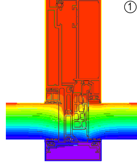
İÇE ÇİFT EKSEN AÇILIM KAPAKLI CEPHE ( TILT&amp;TURN OPENING FACADE WITH CAP )
